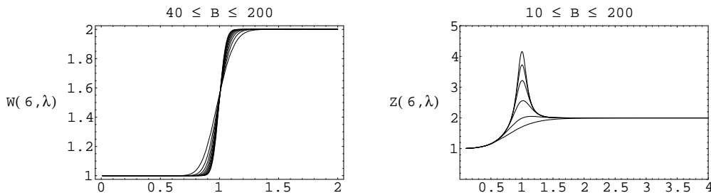
Figure 2: \lambda dependence of the Witten index and the partition function, at \beta = 6 for different cutoffs.
