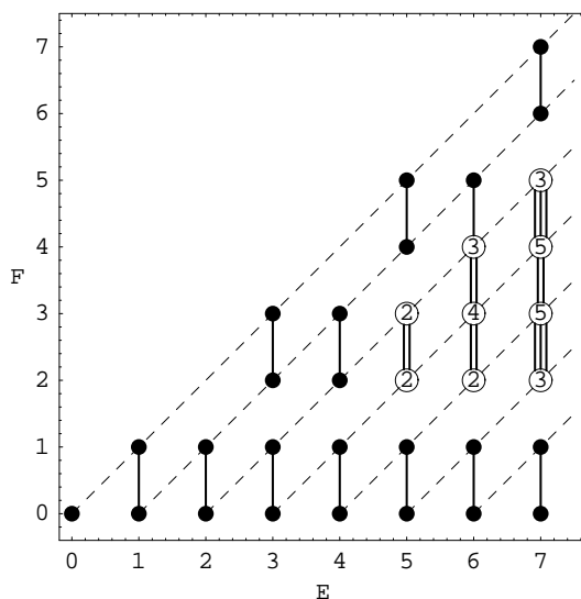
Figure 3: Chew-Frautschi-like plot of the lowest seven levels with their respective degeneracy and supersymmetry partnership at vanishing \lambda .
